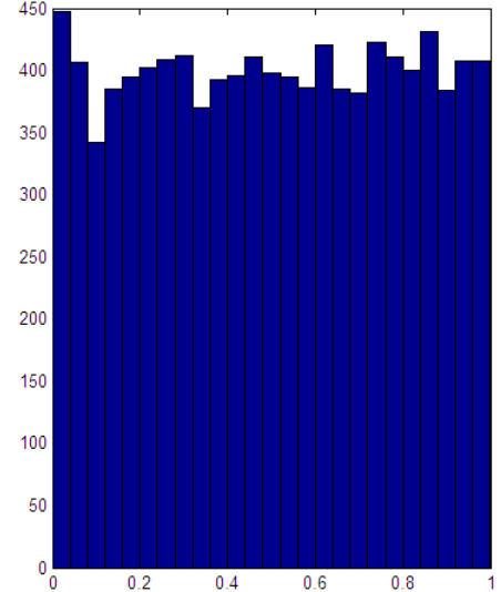
Uniformly Distributed Random Numbers
