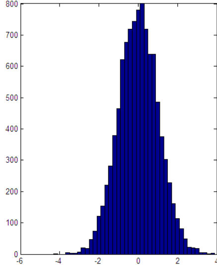
Normally Distributed Random Numbers
